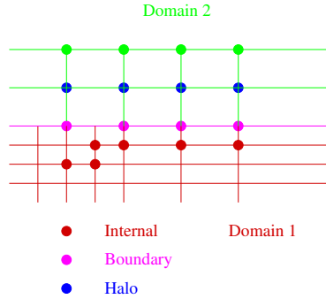
Figure 2: Point classification.
