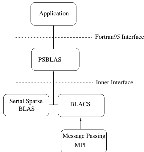
Figure 1: PSBLAS library components hierarchy.
